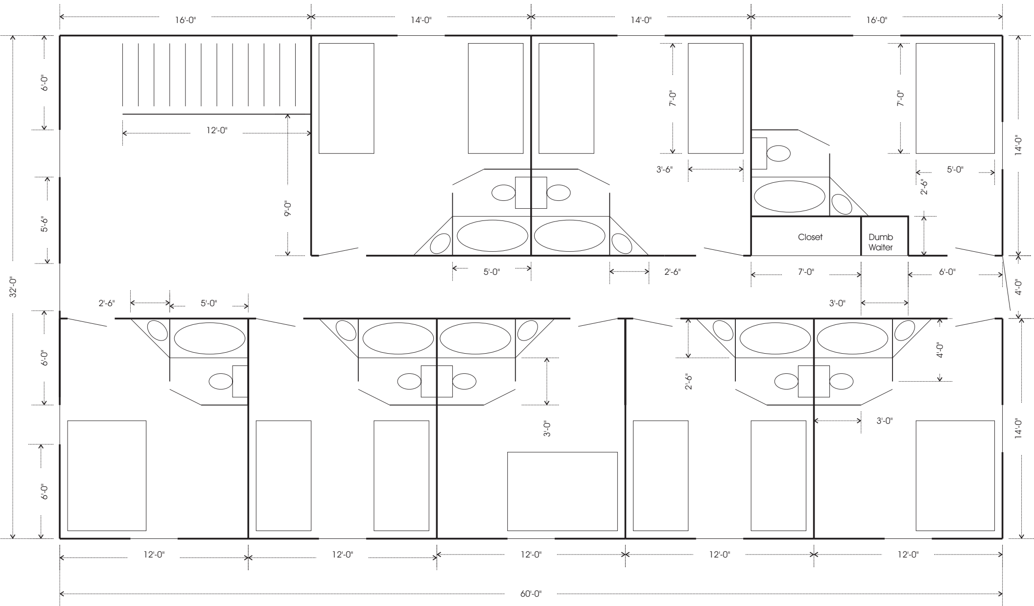
History Ranch Lodge - Second Floor - Revised 9/21/2000
