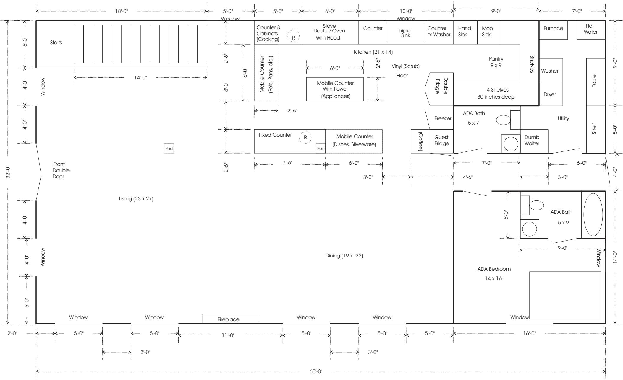
History Ranch Lodge - First Floor - Revised 9/21/2000
